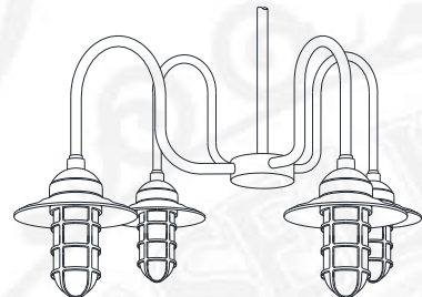
4DPE3 H - 18" W - 40" 3" GLASS & 3" GUARD AVAILABLE FOR 4DPE3
